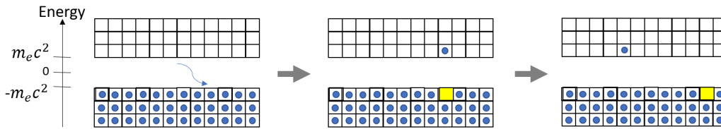
Figure 1 When electrons fill the sea of negative energy states uniformly (left image), those electrons are undetectable. But then the light beam in the left image knocks one of those electrons into a positive energy state (middle image), leaving behind an unfilled negative energy state. A moment later (right image), the positive energy electron and the hole have moved off in different directions. The former appears as a normal electron. The hole appears to be a positive energy, positively charged particle: a positron.
